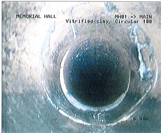
Photo: A_26_07_2013_27_4a.jpg, 00:00:00 5.54m, Circumferential Fracture, from 12 to 12 o'clock
