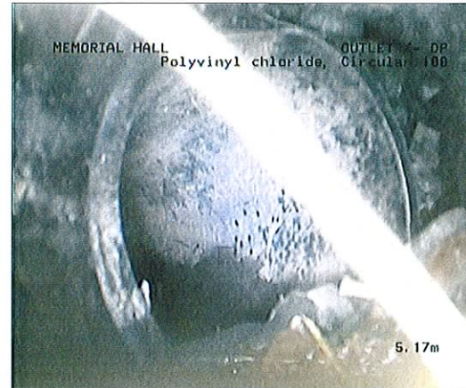
Photo: A_26_07_2013_49_8a.jpg, 00:00:00 5.16m, Joint displaced. Large
