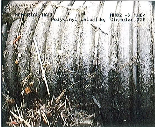
Photo: A_26_07_2013_38_4a.jpg, 00:00:00 0m, Obstruction, 90 % height/diameter loss Remarks: PVC PIPE
