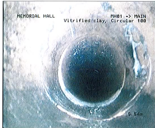
Photo: 3_1_5_08082013_161726_A.jpg, 00:00:00 5.54m, Fine Roots
